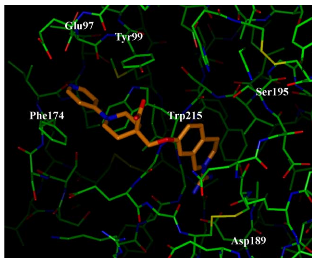
Figure 2. Complex model of factor Xa (green) and compound 1 (orange).
