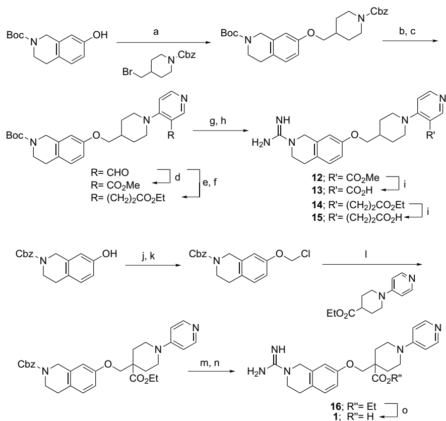
Scheme 2. Synthesis of compounds 1 and 12–16 . Reagents and conditions: 6 (a) NaH, DMF, rt; (b) H 2 (3 atm), 7.5% Pd/C (cat.), THF–EtOH, rt; (c) 4-chloro-3-formylpyridine, Et 3 N, EtOH, reflux; (d) MnO 2 , NaCN (cat.), CHCl 3 –MeOH, rt; (e) (EtO) 2 POCH 2 CO 2 Et, NaH, THF, rt; (f) H 2 (1 atm), 7.5% Pd/C (cat.), THF–EtOH, rt; (g) TFA, CHCl 3 , rt; (h) 1 H -pyrazole-1-carboxamide hydrochloride, DIPEA, DMF, rt; (i) NaOH, MeOH–H 2 O, rt, then HCl aq; (j) ClCH 2 SMc, NaH, DMF, rt; (k) SO 2 Cl 2 , CH 2 Cl 2 , 0 °C; (l) LDA, THF, –70 °C rt; (m) 30% HCl–EtOH, 85 °C; (n) 1 H -pyrazole-1-carboxamide, NaHCO 3 aq, acetone, rt; (o) c-HCl, reflux.
