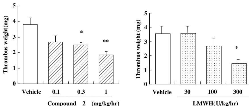
Figure 4. Effect of compound 2 and LMWH on venous thrombosis in rats. (Data represent the mean \pm SEM, ** P < 0.01, * P < 0.05, Dunnett's test, n = 5–7). 12
