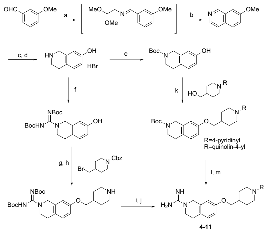
Scheme 1. Synthesis of compounds 4–11 . Reagents and conditions: 6 (a) aminoacetal, toluene, reflux; (b) 76% H 2 SO 4 aq, 0°C; (c) H 2 (3 atm), PtO 2 (cat.), AcOH, rt; (d) HBr aq, reflux; (e) Boc 2 O, NaOH, dioxane–H 2 O, rt; (f) 1 H -pyrazole-1-( N,N' -bis- tert -butoxycarbonyl) carboxamidine, Et 3 N, THE, rt; (g) NaOH, DMSO, rt; (h) H 2 (3 atm), 7.5% Pd/C (cat.), THF–EtOH, rt; (i) ethyl acetoimidate hydrochloride, Et 3 N, THF–EtOH, rt for 5 ; nitro-benzyl bromide, diisopropylethylamine (DIPEA), THF–DMF, rt, then H 2 (3 atm), 7.5% Pd/C for 6 and 7 ; picolyl chloride, DIPEA THF–DMF, rt for 8 and 9 ; (j) TFA, CHCl 3 , rt, then HCl–MeOH; (k) diisopropyl azodicarboxylate (DIPAD), PPh 3 , THE, rt; (l) TFA, CHCl 3 , rt; (m) 1 H -pyrazole-1-carboxamidine hydrochloride, DIPEA, DMF, rt, then HCl–MeOH for 10 and 11 .
