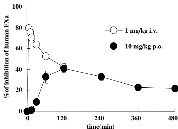
Figure 3. Percent inhibition of human factor Xa after intravenous and oral administration of compound 2 to cynomolgus monkeys. 10 Data represent the mean \pm SEM ( n = 6 ).
